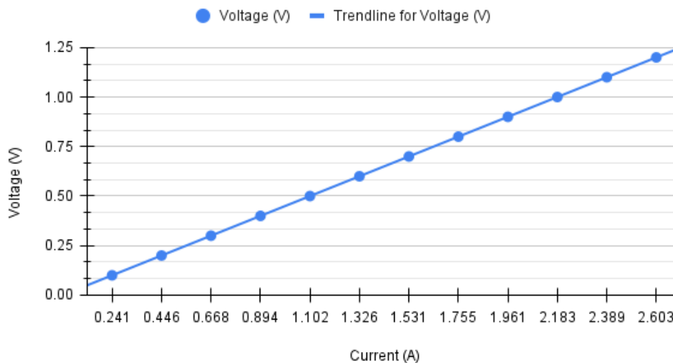
Current (A) vs. Voltage (V)
