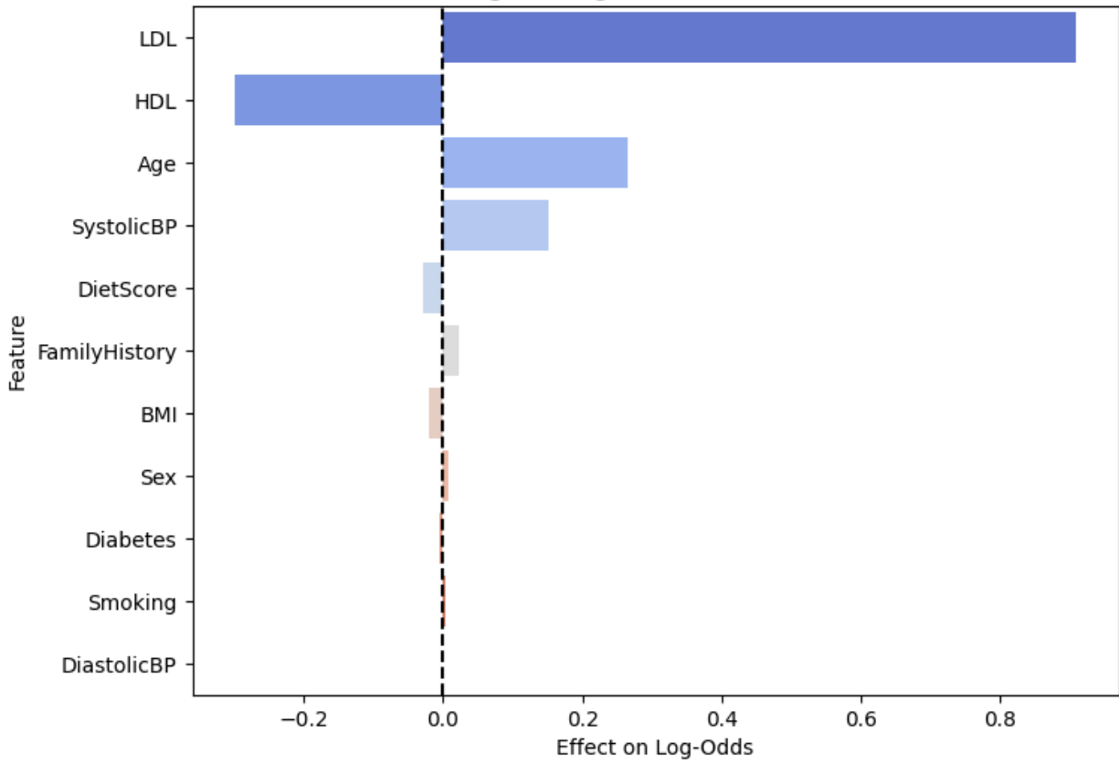
Feature Influence on Severe CAD Prediction (Logistic Regression Coefficients)
