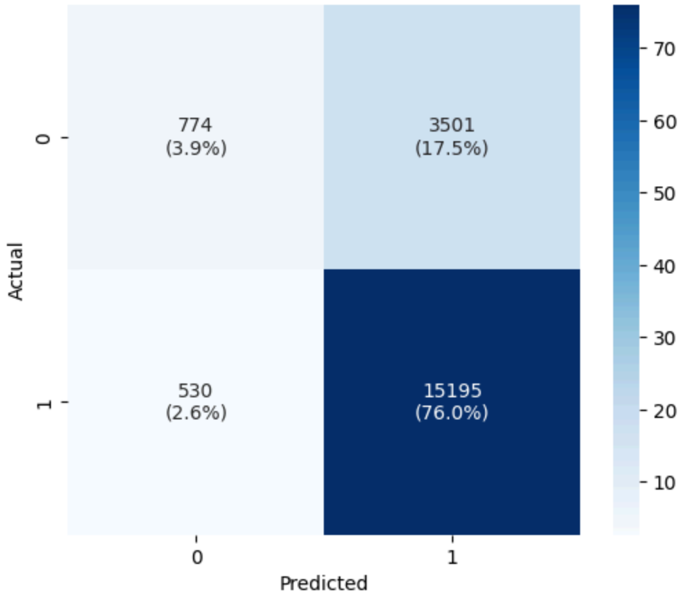
Confusion Matrix Counts and Percentage of Total Predictions
