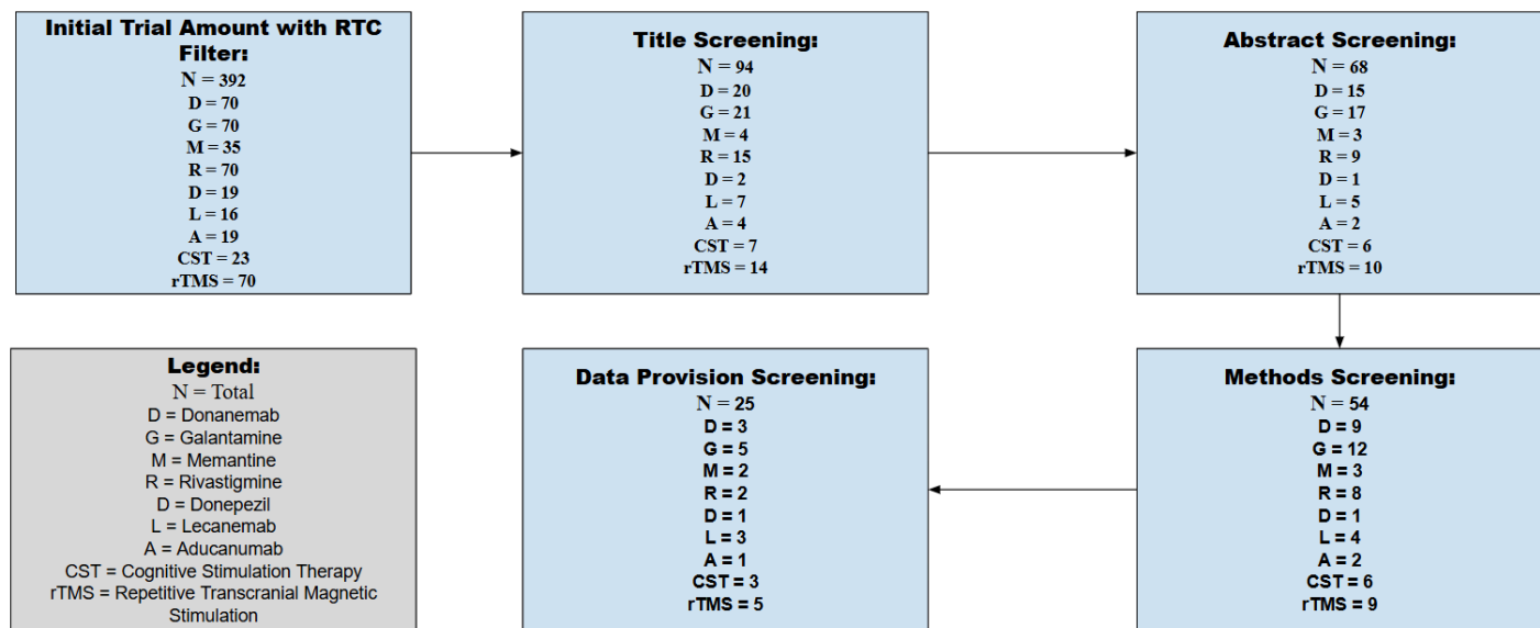
Figure 1. A flow chart depicting the number of trials at each filter (n = total) after each filter.
