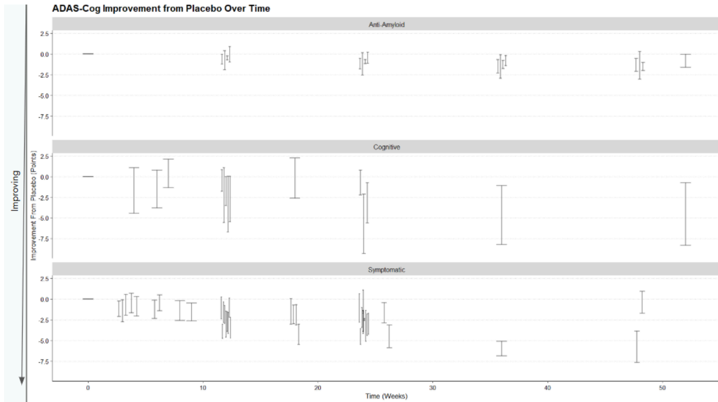
Figure 6.1 is a facet wrapped scatterplot of the impact of three treatment types (anti-amyloid, symptomatic, and cognitive therapy) on the ADAS-Cog score over time. All treatments improved by some amount over time compared to the placebo. Symptomatic treatments have a larger regression slope, indicating larger improvement over the same timeframe and more variation compared to anti-amyloid treatments. Anti-amyloid treatments have very consistent improvement with little variation compared to the other treatment types. Cognitive treatments have a lot of variation between datapoints, shown by the large error bars.
