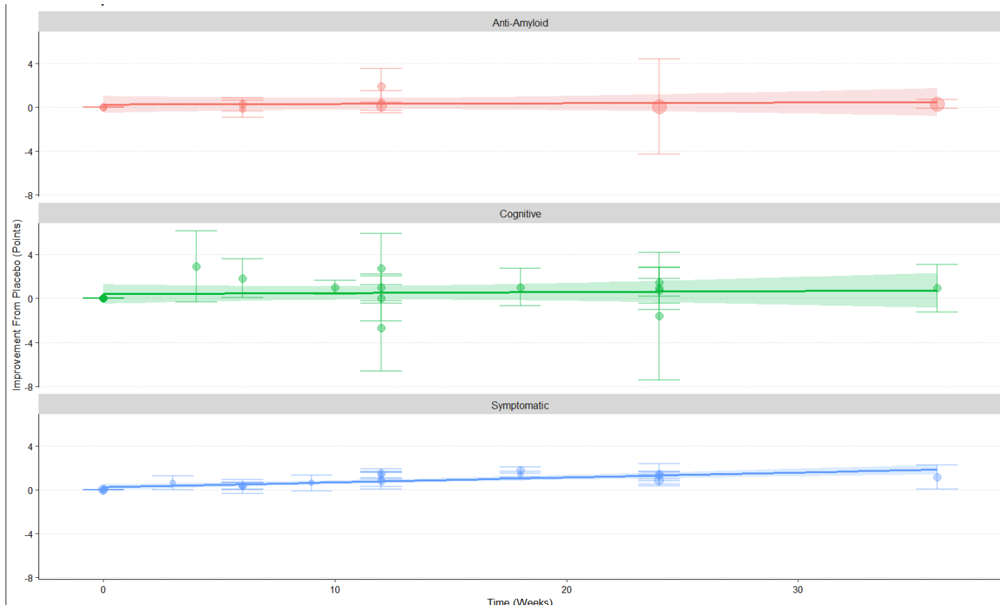
Figure 5.1 Jittered facet wrapped scatterplot of three different treatment types effect on ADAS-Cog
